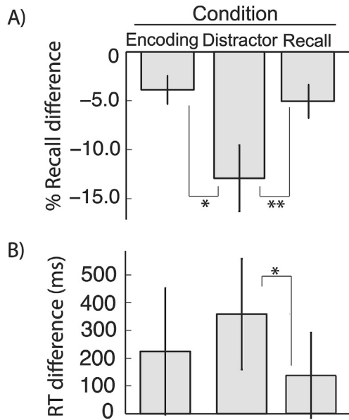
Fig. 2. A. Probability of recall across stimulation conditions. Across-electrode mean and \pm 1SEM of normalized probability of recall for each stimulation condition. Stimulation condition modulated probability of recall ( MSE = 0.019, F_{2,23} = 5.97, p = 0.013 ) and stimulation during distractor led to worse recall than stimulation during encoding ( t_7 = 2.53, p = 0.039 ) and retrieval ( t_7 = 3.78, p = 0.007 ). We did not find a difference in probability of recall during encoding and retrieval periods ( t_7 = 0.79, p = 0.789 ). B. Response time across stimulation conditions. Across electrode mean and \pm 1SEM of normalized response times for each stimulation condition. There was a strong trend towards stimulation condition modulating response time ( MSE = 99.1 \times 10^3, F_{2,23} = 3.31, p = 0.067 ). Stimulation during the arithmetic distractor led to slower recall than stimulation during retrieval ( t_7 = 2.81, p = 0.026 ), and a comparison between distractor-period stimulation and encoding stimulation trended in the same direction ( t_7 = 1.85, p = 0.106 ). We did not identify a difference between response times during encoding or distraction conditions ( t_7 = 0.83, p = 0.440 ). In both panels, single and double asterisks mark significance, respectively p < 0.05 and p < 0.01 .
