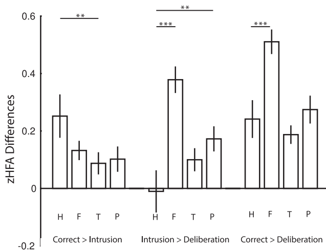
Figure 2. Retrieval Contrasts
